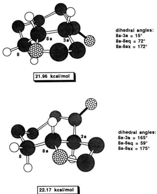
Figure 1. Minimum energy conformations for cis - and trans -octahydrocyclohepta[ b ]furan-4-ones (MMX force field, only hydrogens at C(3a), C(8a), and C(8) are shown).
