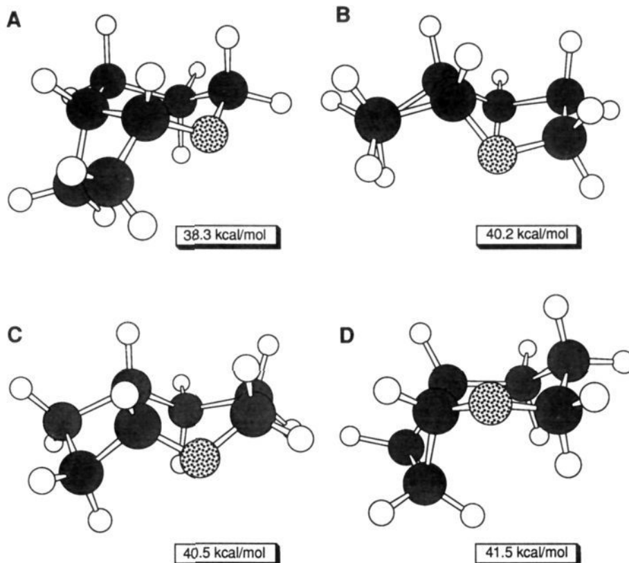
Figure 5. Four lowest energy conformations of cis -2-oxabicyclo[4.2.0]octane as determined by molecular mechanics calculations (MMX force field).
