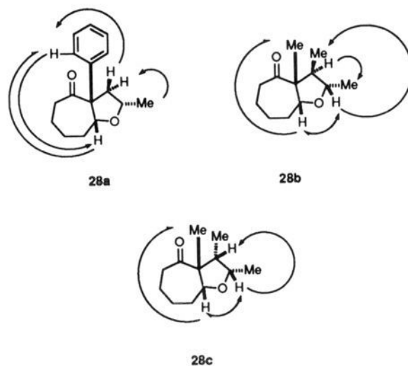
Figure 2. Key ^1\text{H} NOE enhancements for cycloheptafuranones 28 .
