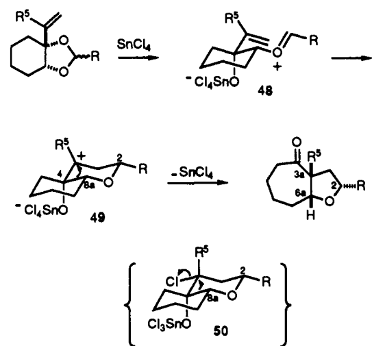
Scheme VIII
