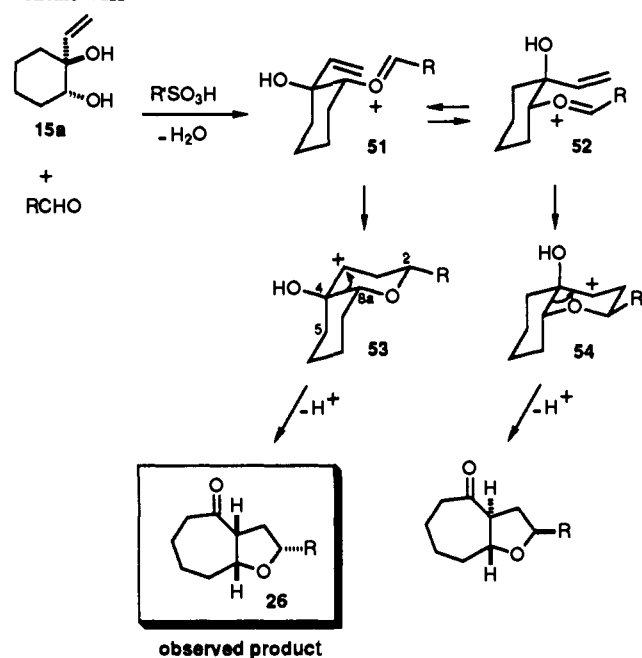
Scheme VIII
