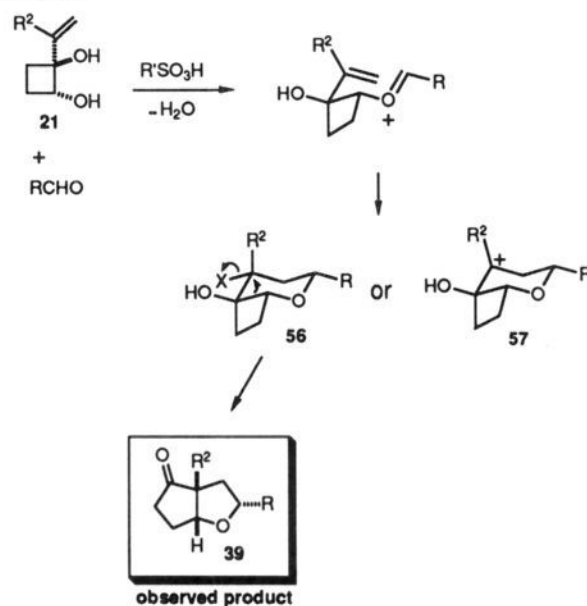
Figure 5. Four lowest energy conformations of cis -2-oxabicyclo[4.2.0]octane as determined by molecular mechanics calculations (MMX force field).
