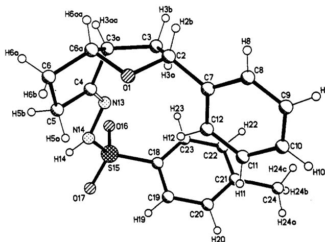
Figure 3. View of the crystallographic model of 40 .
