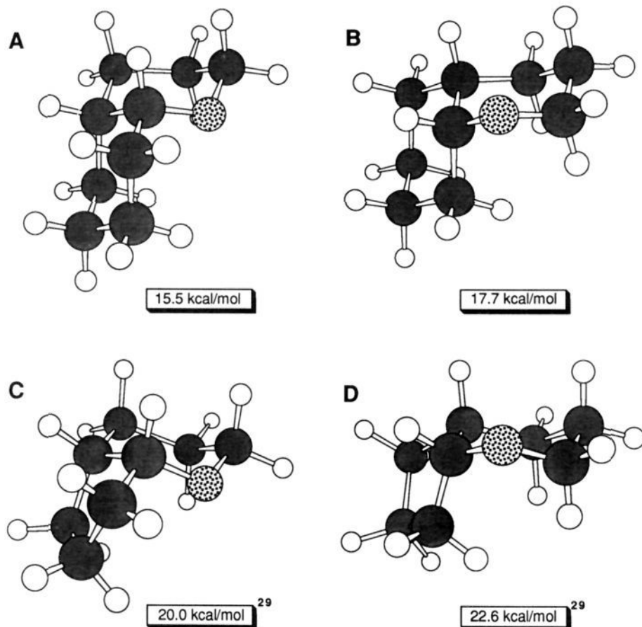
Figure 4. Lowest energy chair hydroxypryan conformations of cis -octahydro-2 H -1-benzopyran (A and B) and cis -2-oxabicyclo[4.2.0]nonane (C and D) as determined by molecular mechanics calculations (MMX force field).
